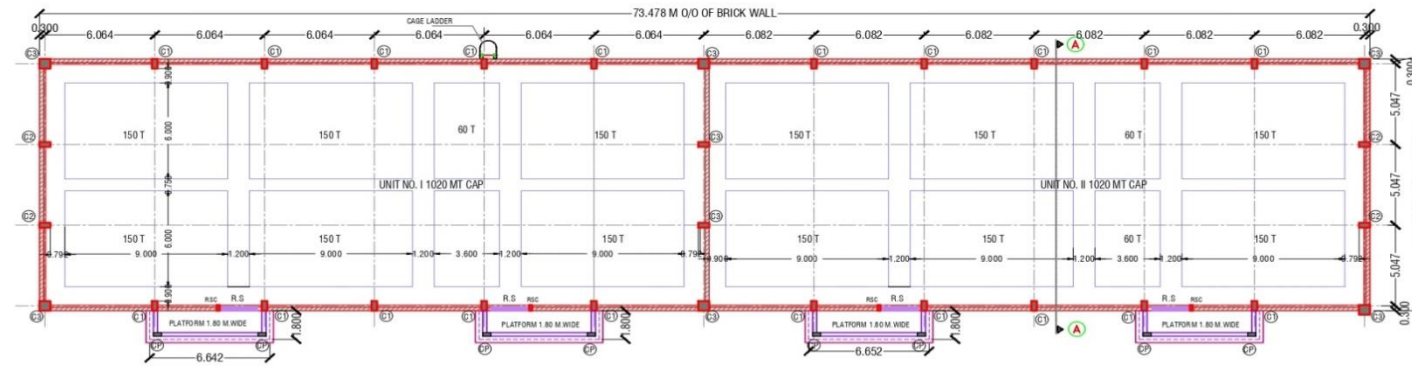
PLAN FOR 2040 MT.WH. UNIT NO. I & II
